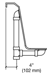
PLUMBING ROUGH-IN
