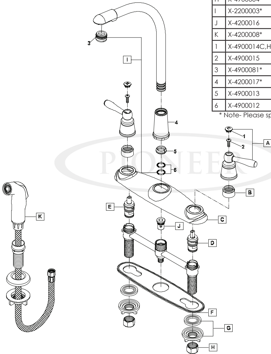
Product Diagram
