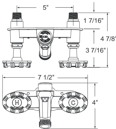
Model 122 Rough-In Dimensions
