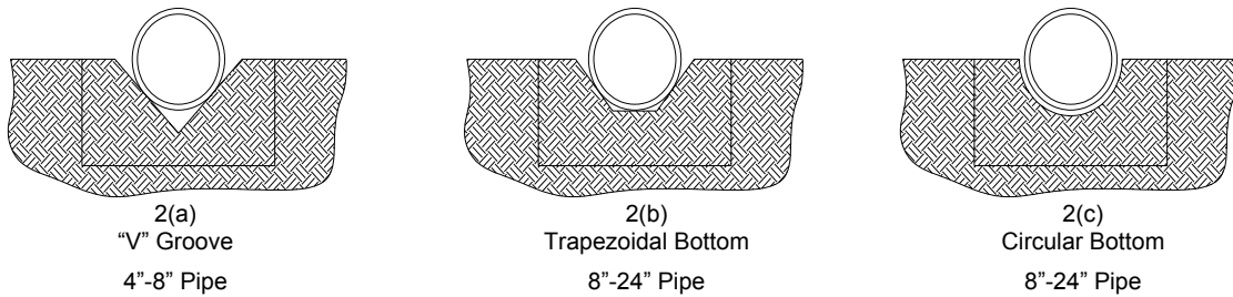
Figure 2 Shaped Trench Bottoms
