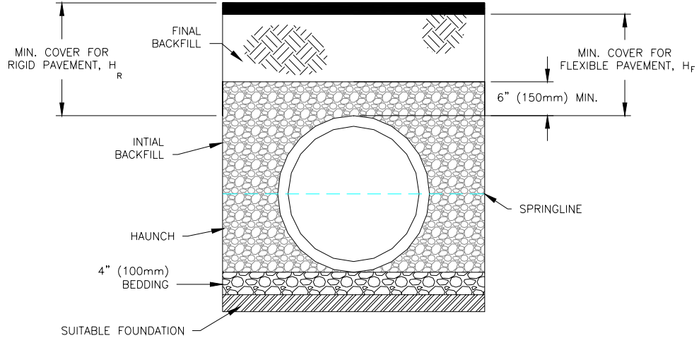
Figure 1 Typical Backfill Structure
