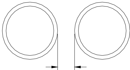
12" (300mm) FOR 3"-24" (75-600mm) PIPE
