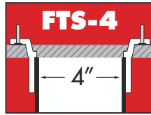
4" Flange on 4" Drain Pipe
