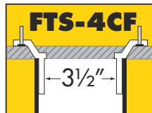
3x4 Flange / Slab Flange in 4" Drain Pipe
