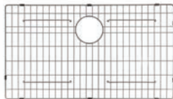
KBG-100-32 ..... Bottom Grid 29 9/16" x 16 9/16" x 1 3/8" Stainless Steel Included with KHU100-32 or sold separately
