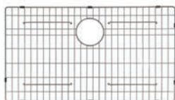
KBG-200-30 ..... Bottom Grid 27 1/2" x 15 11/16" x 1 3/8" Stainless Steel Included with KHF200-30 or sold separately
