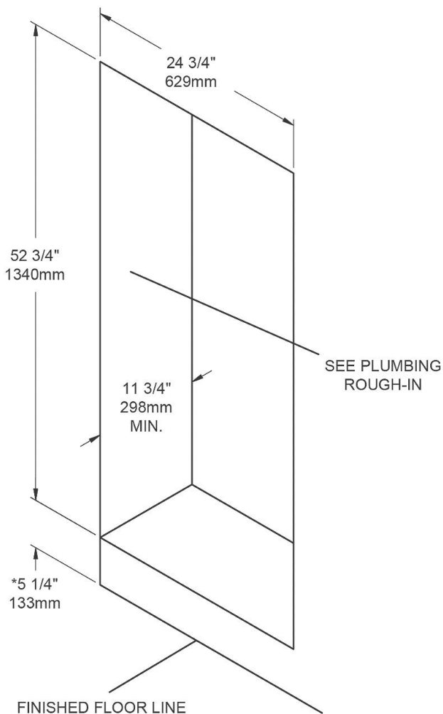
MB23A Mounting Box Installation Fountain with Cup Dispenser
