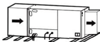
Horizontal Right Configuration - Must Relocate Drain Pan
