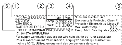
Fig. Example of nameplate, ALPHA 15-55 HWR-D models
