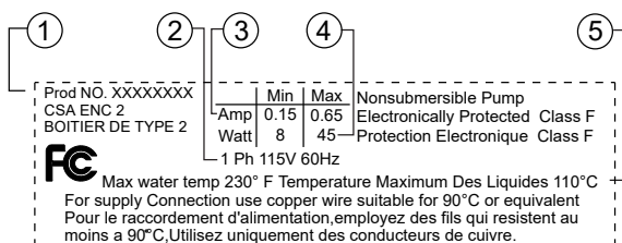
Fig. Example of nameplate, ALPHA1
