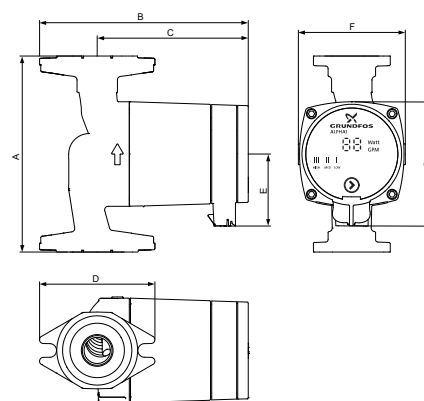
ALPHA1 15-55 FR line cord
