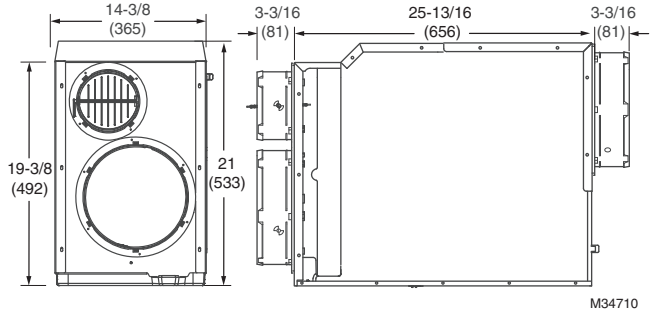
DR120A dimensions in Inches (millimeters)
