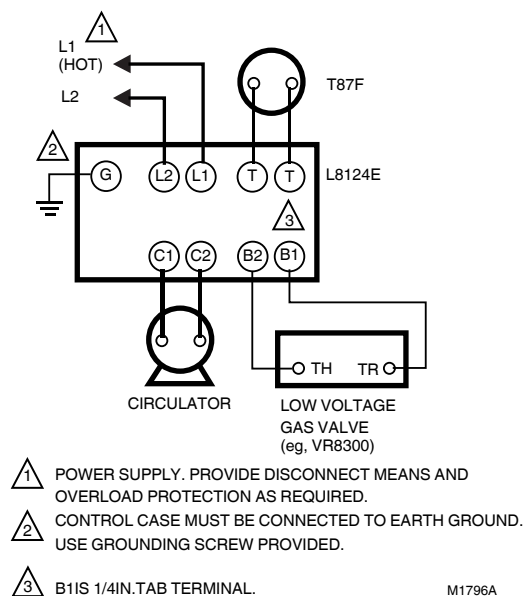
Fig. 14. L8124E in a 24V, gas-fired forced hot water, tankless system.
