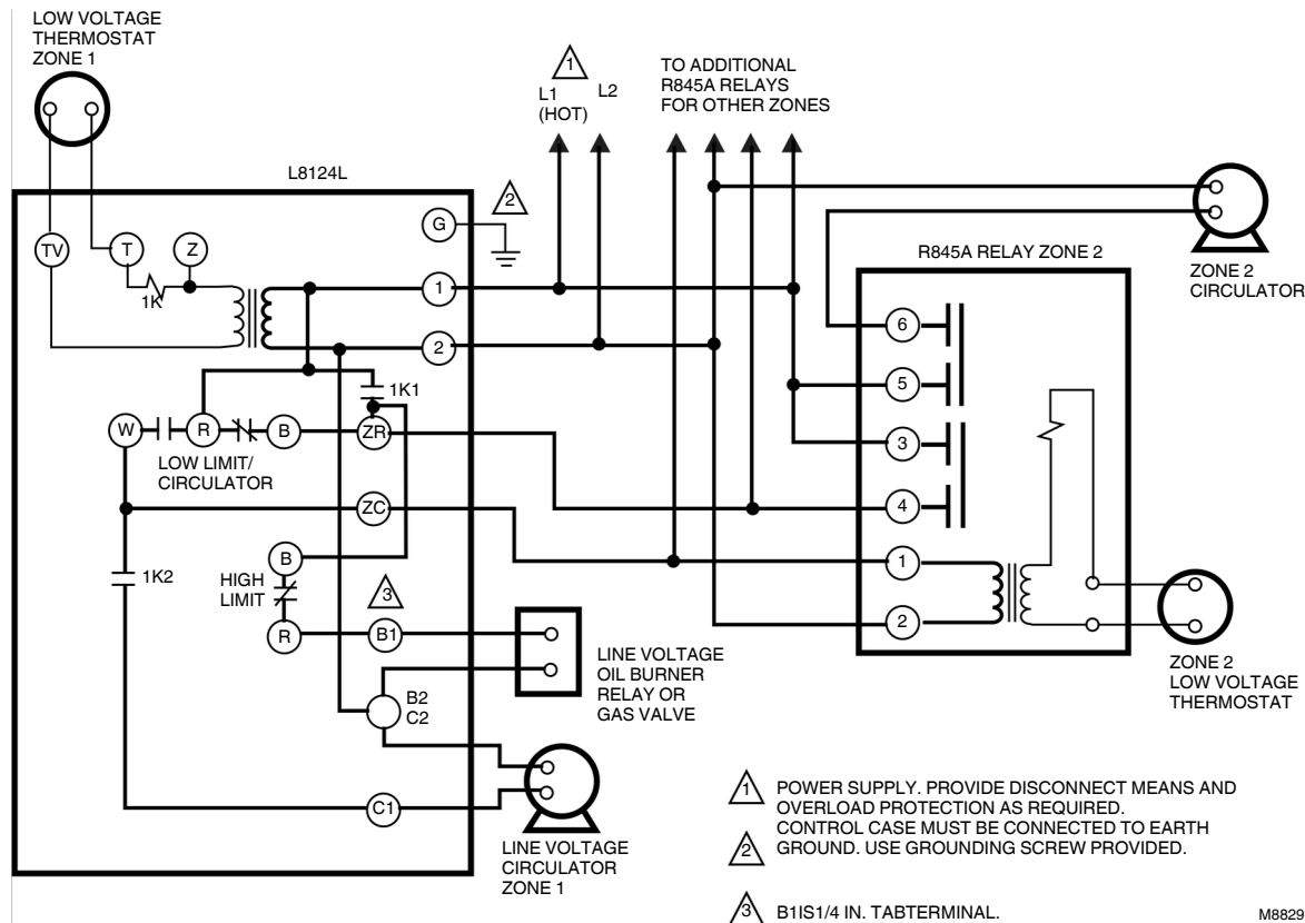
Fig. 20. L8124L multizone system with circulator connections and internal schematic.
