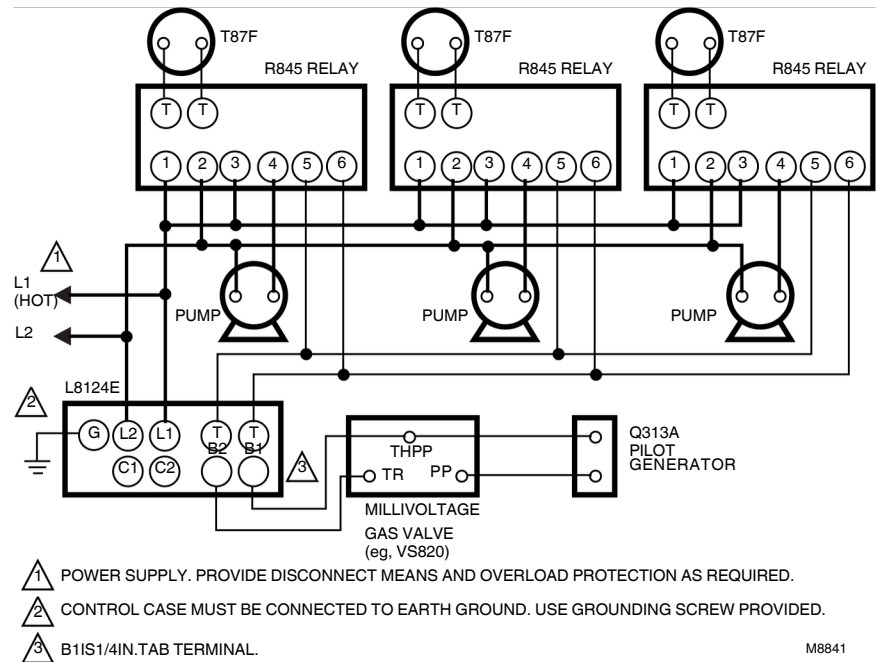
Fig. 12. L8124B in a gas-fired, millivolt, forced hot water, tankless, zoned, pump system.
