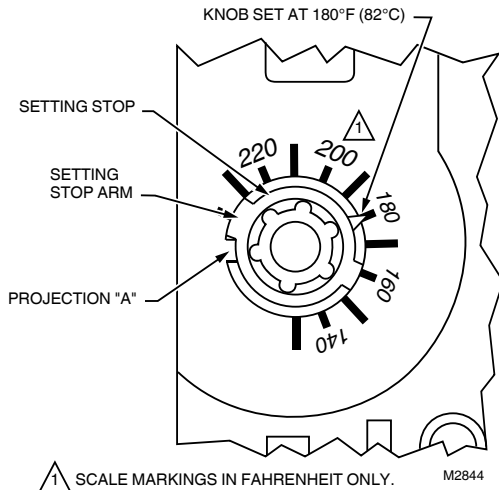
Fig. 22. Setting stop in position to limit the high limit setting to 200°F (93°C).
