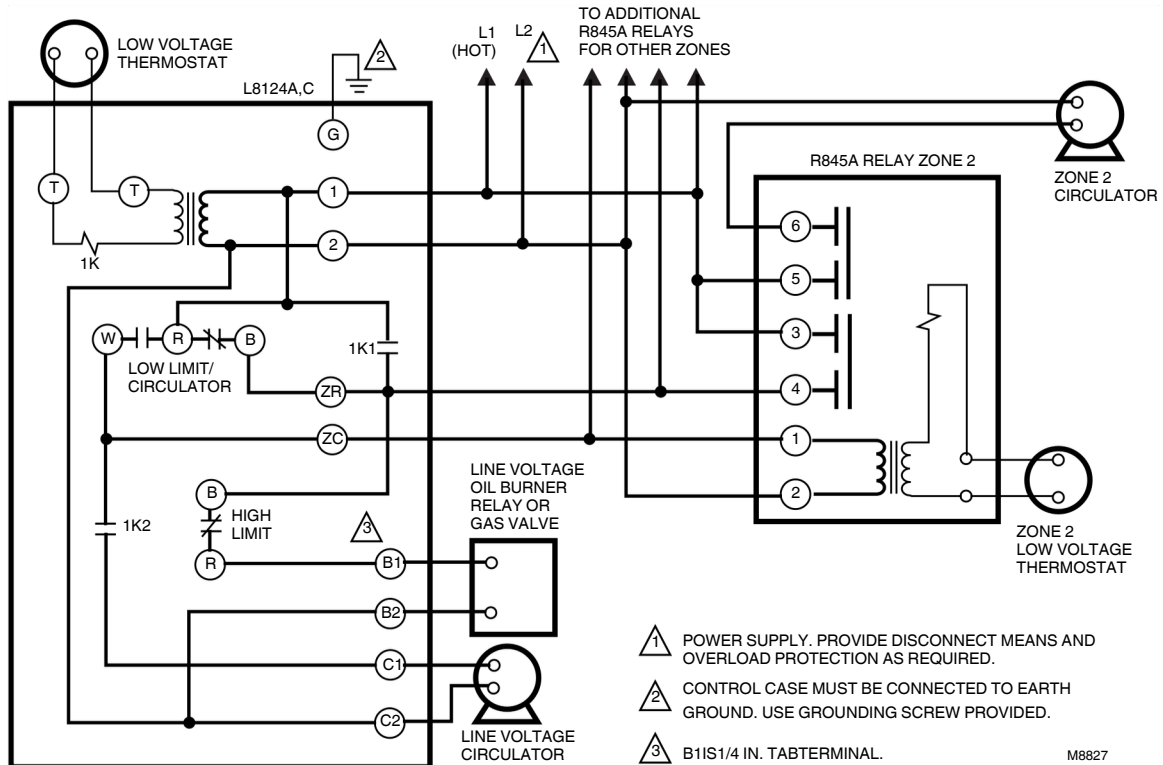
Fig. 18. L8124A,C multizone system with circulator connections and internal schematic.
