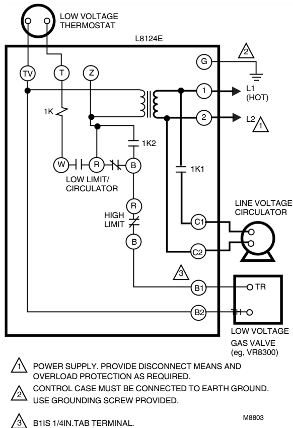
Fig. 13. L8124E single zone connections and internal schematic.
