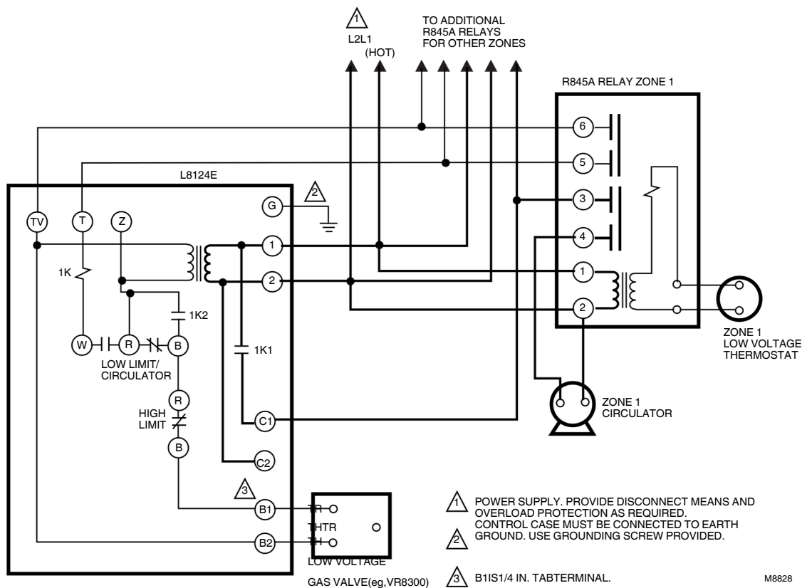
Fig. 19. L8124E multizone system with circulator connections and internal schematic.
