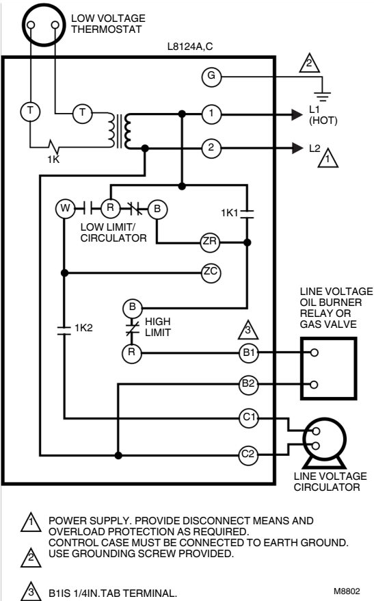
Fig. 9. L8124A,C single zone connections and internal schematic.
