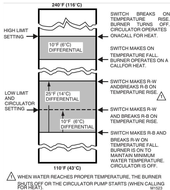
Fig. 21. Relationship of set points and differential.
