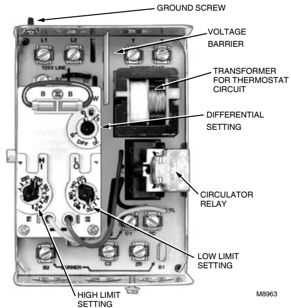
Fig. 7. Internal view of L8124M.
