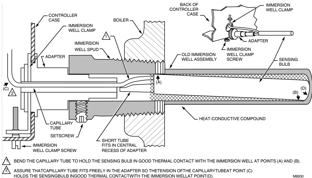
Fig. 8. Position of bulb in immersion well, and use of well adapter when required.
