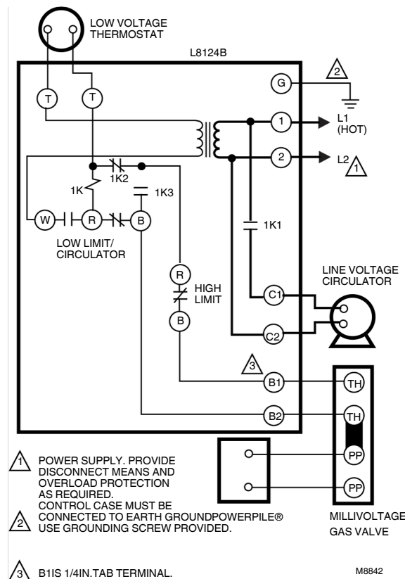
Fig. 11. L8124B single zone connections and internal schematic.
