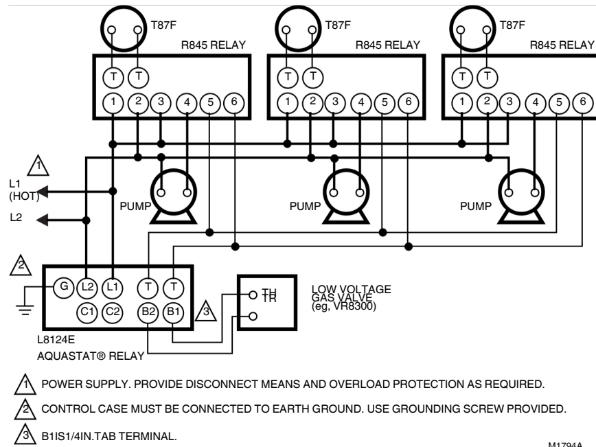
Fig. 15. L8124E in a 24V, gas-fired forced hot water, tankless, zoned pump system.
