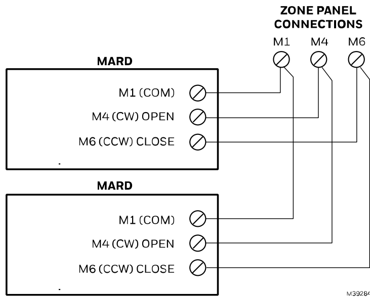
Figure 2. Wiring two MARDs in tandem to a zone panel.
