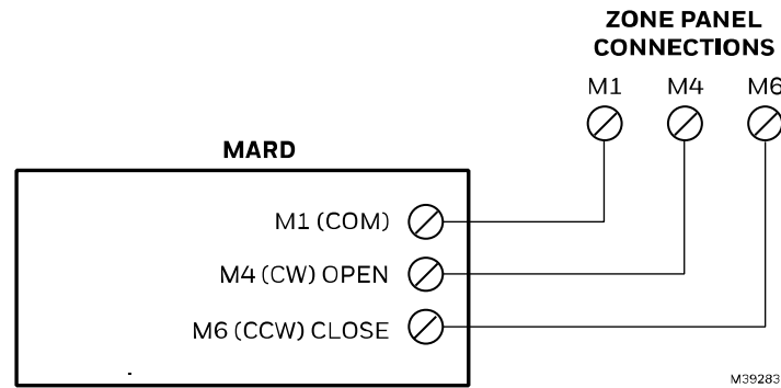
Figure 1. Wiring a MARD to a Conventional Zone Panel
