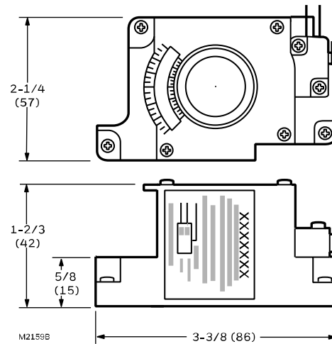
Figure 9. Dimension Drawing
