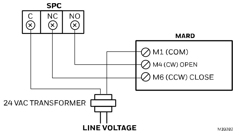
Figure 3. Wiring SPC to control MARD damper in bypass applications
