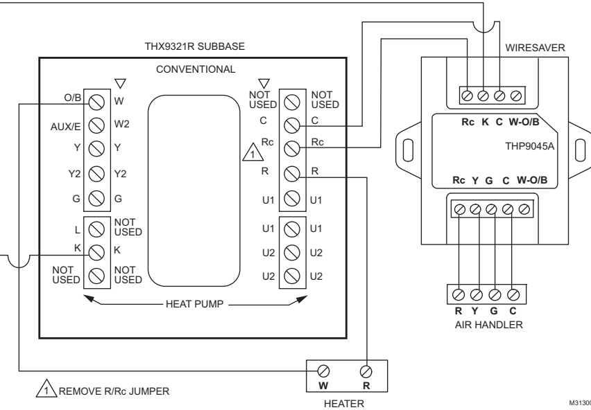
Fig. 4. Example wiring diagram for a 1H/1C system with 2 transformers.
