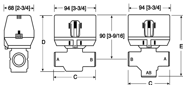
Fig. 1. Nominal dimensions in inches [millimeters]
