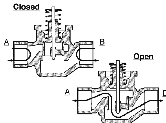
Fig. 2. Fluid Flow of 2-way valves
