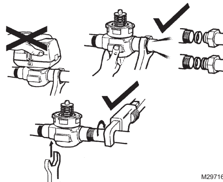
Fig. 4. Plumbing of the VC Valve
