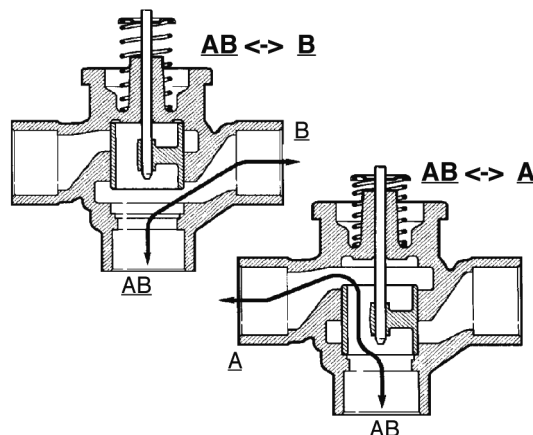
Fig. 3. Fluid flow of 3-way valves
