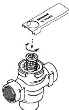
Fig. 5. Installing Cartridge
