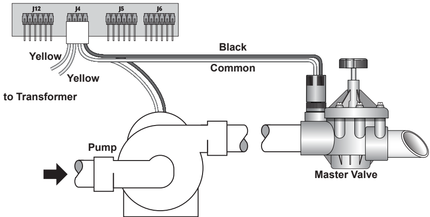
Figure 6 – Master Valve and Pump Electrical Connections
