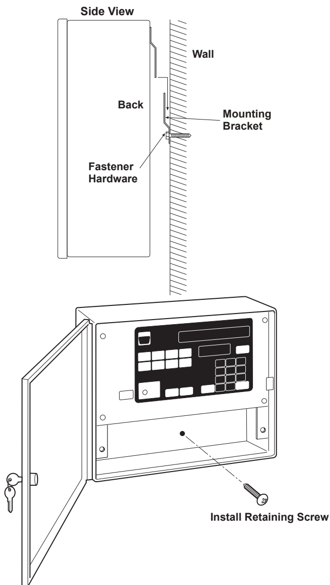
Figure 3 – Controller Mounting
