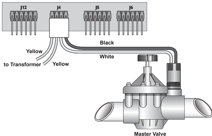
Figure 5 - Master Valve Electrical Connection
