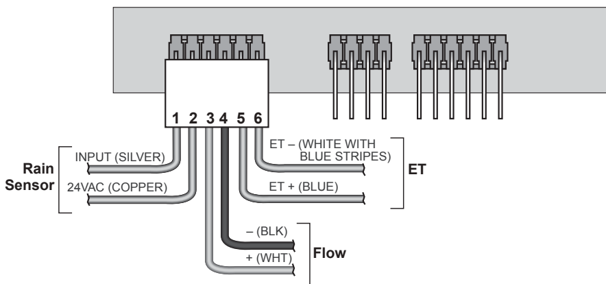
Figure 11 – Sensor Interface Electrical Connections
