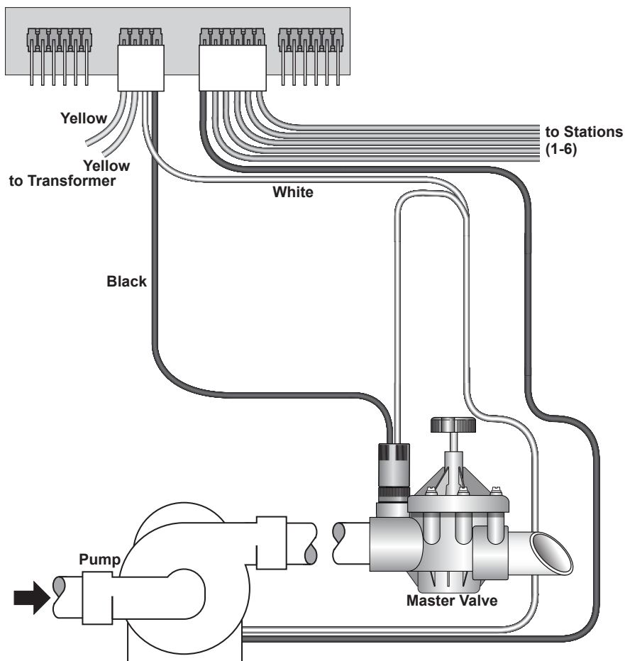
Figure 9 - Normally Open Master Valve and Pump
