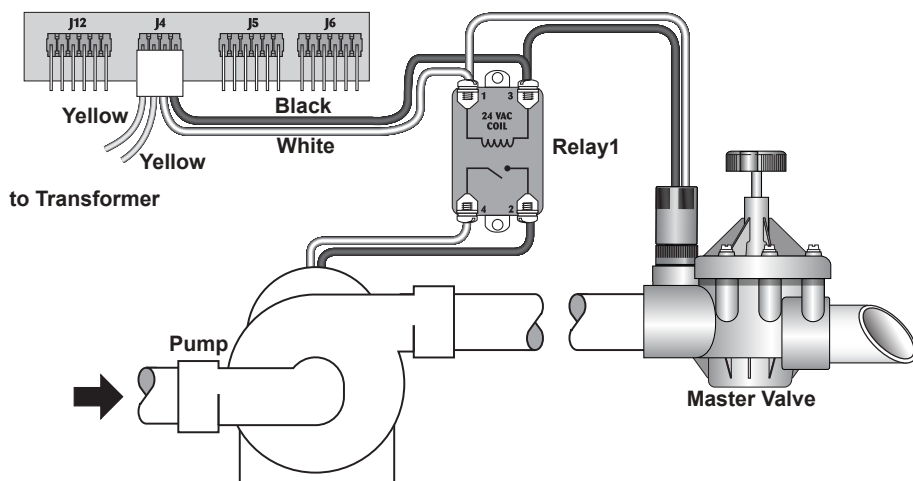
Figure 7 – Master Valve and Pump Electrical Connections with Isolation Relay
