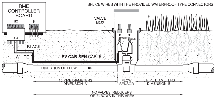
Figure 10 - Flow Sensor Electrical Connections
