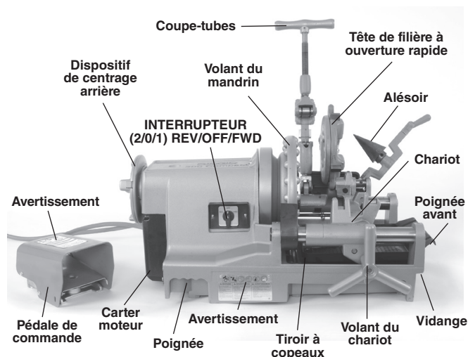
Figure 1 – Fileteuse 300 Compact
