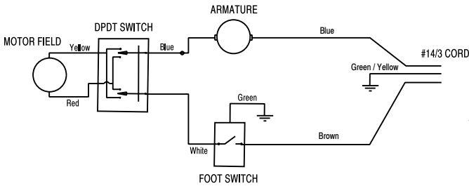
5401TMSO (240 Volt) Wiring Schematic
