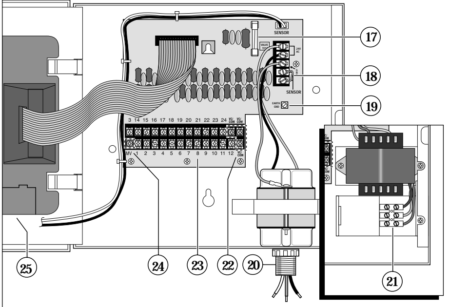
Controller Components
